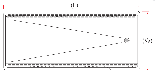
Top View Model : ATVA-2-D (With downdraft)
